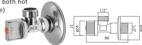
Quarter turn angle valve
