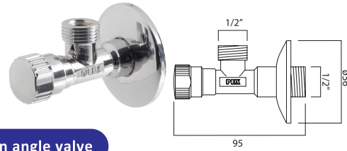
Quarter turn angle valve
